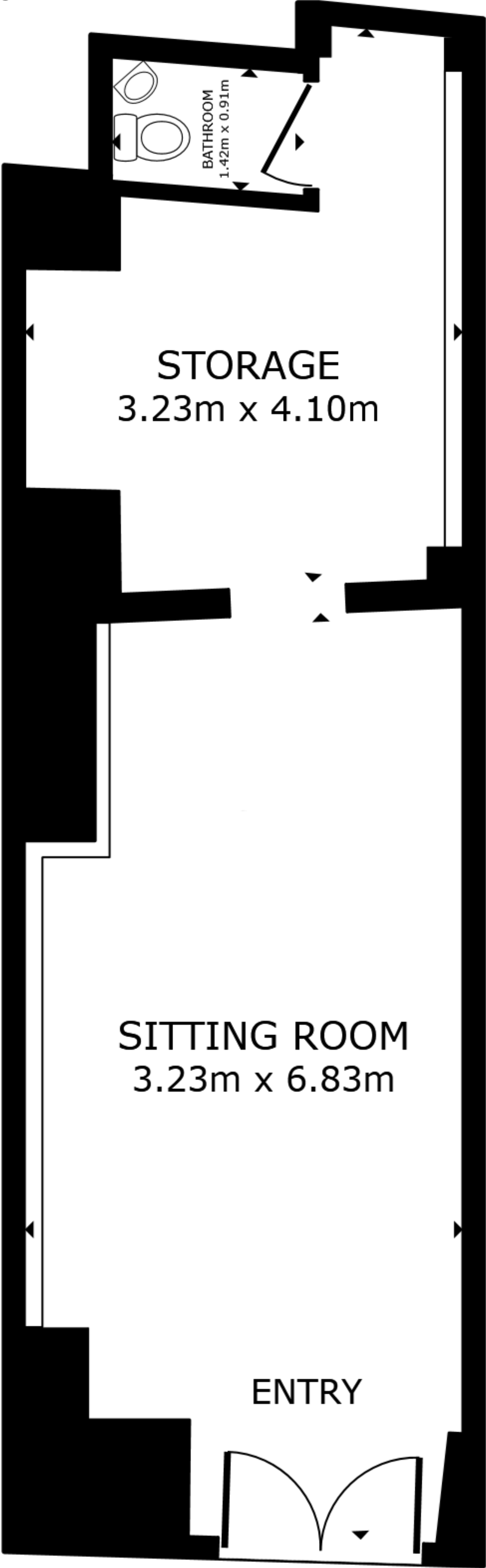
FLOOR PLAN
